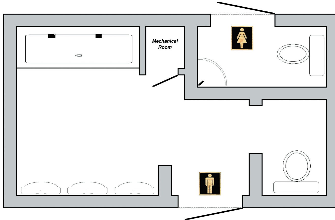
Typical Layout for Trailer-mounted Washrooms (13' x 8')
