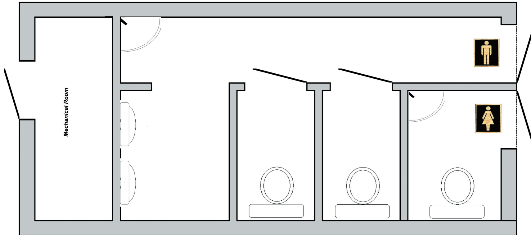
Typical Layout for Skid-mounted Washrooms (16' x 8')
